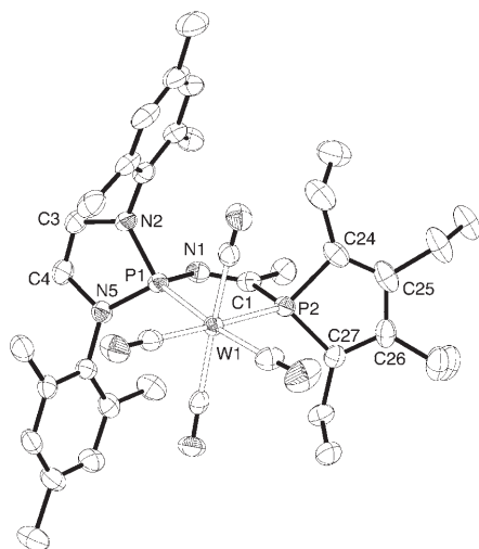
Figure 1. Molecular structure of 3a in the solid state (H atoms omitted; 50% probability thermal ellipsoids). Selected bond lengths [Å] and angle [°]: W1–P2 2.450(1), W1–P1 2.459(1), N1–C1 1.270(6), N1–P1 1.766(4), C1–P2 1.888(5), P1–N5 1.688(4), P1–N2 1.692(4), N2–C3 1.418(6), C3–C4 1.327(7), C4–N5 1.417(6), P2–C24 1.803(5), P2–C27 1.807(5), C24–C25 1.354(7), C25–C26 1.466(7), C26–C27 1.365(6); P2–W1–P1 79.33(4).
