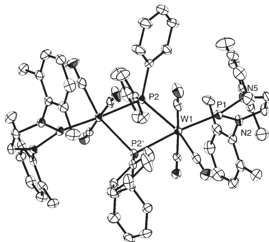
Figure 3. Molecular structure of 6 in the solid state (H atoms omitted; 50% probability thermal ellipsoids). Selected bond lengths [Å] and angles [°]: W1–P1 2.251(2), W1–P2' 2.577(2), W1–P2 2.596(2), P1–N2 1.684(5), P1–N5 1.692(5), N2–C3 1.386(7), C3–C4 1.327(9), C4–N5 1.392(7); P2'–W1–P2 76.9(1), N2–P1–N5 88.5(2), N2–P1–W1 134.4(2), N5–P1–W1 135.7(2), W1'–P2–W1 101.7(1).
