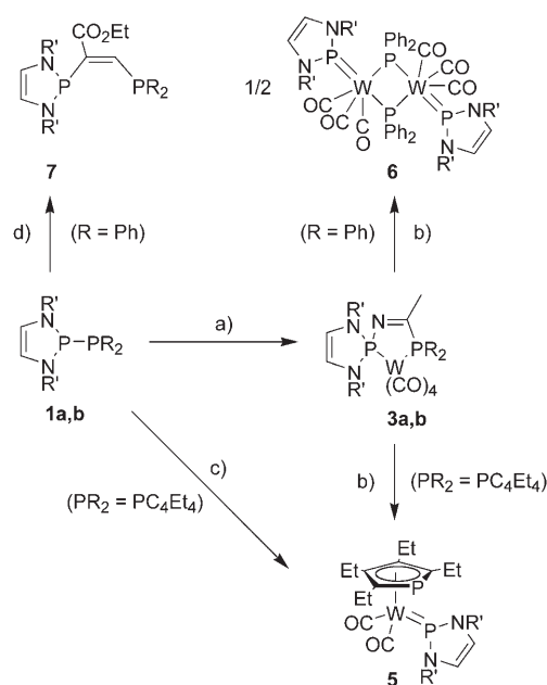
Scheme 1. PR 2 = 2,3,4,5-tetraethylphosphinyl, R' = Mes ( 1a , 3a , 5 ); R = Ph, R' = 2,6-Me 2 C 6 H 3 ( 1b , 3b , 6 , 7 ). Reagents and conditions: a) 1 equiv [W(CO) 4 (cod)] ( 2 ), MeCN, 20 °C (for 1a ) or 50 °C (for 1b ); b) 185 °C; c) 1 equiv [W(CO) 3 (MeCN) 3 ] ( 4 ), 20 °C, toluene; d) 1 equiv ethyl propiolate, toluene, 0–20 °C; cod = cycloocta-1,5-diene, Mes = 2,4,6-Me 3 C 6 H 2 .
