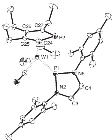
Figure 2. Molecular structure of 5 in the solid state (H atoms omitted; 50% probability thermal ellipsoids). Selected bond lengths [Å] and angles [°]: W1–P1 2.218(1), W1–C25 2.362(4), W1–C26 2.371(3), W1–C24 2.381(4), W1–C27 2.398(3), W1–P2 2.560(1), W1–centroid(C 4 P) 2.014(2), P1–N5 1.681(3), P1–N2 1.684(3), N2–C3 1.405(4), C3–C4 1.333(4), C4–N5 1.391(4); N5–P1–N2 88.7(1), N5–P1–W1 134.0(1), N2–P1–W1 137.0(1).
